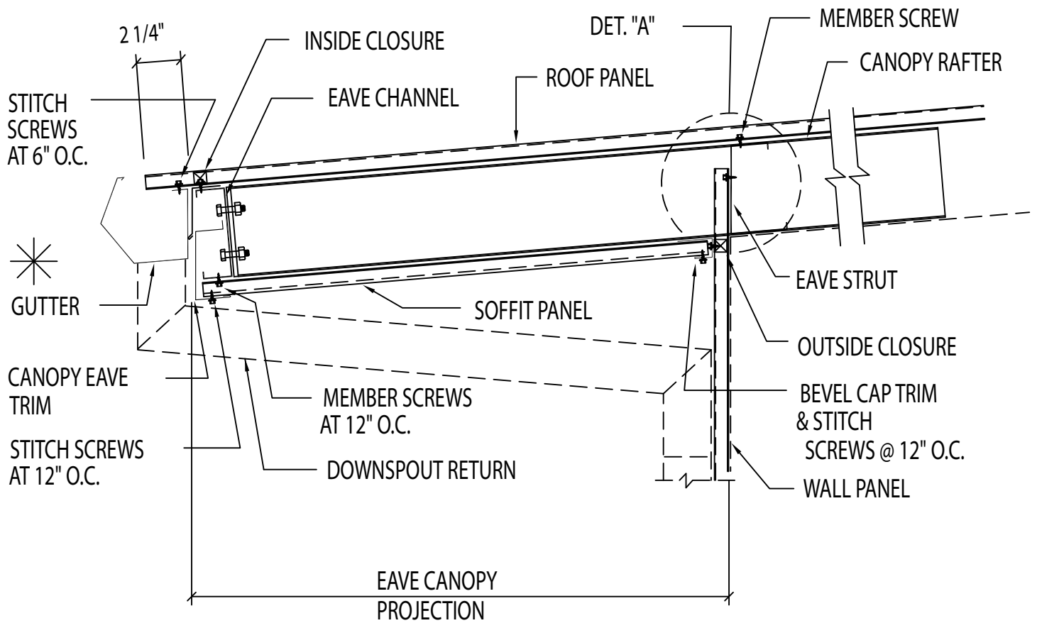
FLUSH EAVE LINE CANOPY WITH SOFFIT PANEL
