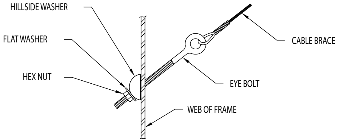
CABLE BRACE TO FRAME DETAIL
