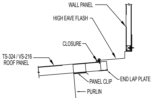
TS-324 / VS-216 HIGH LOW EAVE DETAIL
